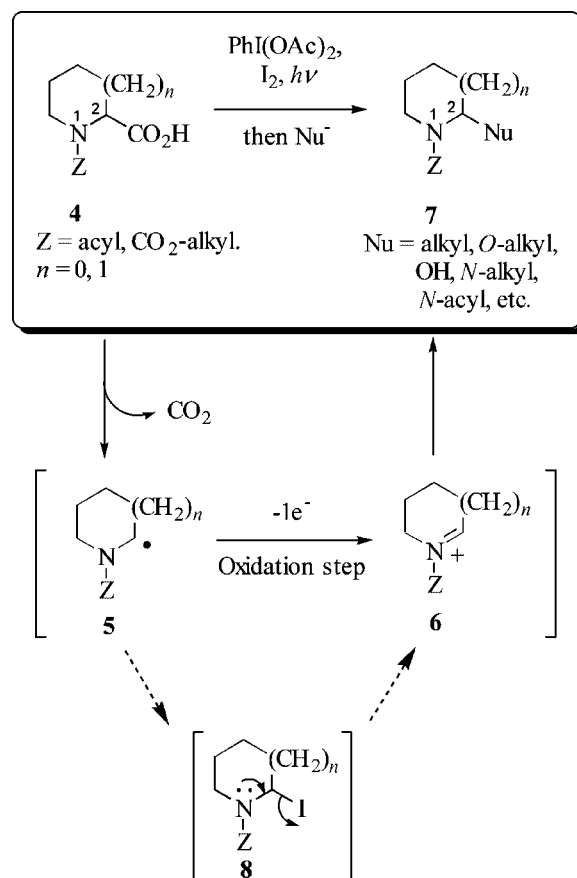
Scheme 1. Synthesis of substituted nitrogen heterocycles from \alpha -amino acids
