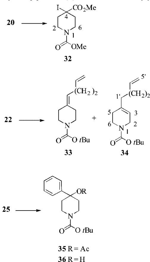
Scheme 7. Synthesis of functionalized nitrogen heterocycles by radical decarboxylation of 4-substituted \beta - and \gamma -amino acids; see Table 2 for conditions and yields
