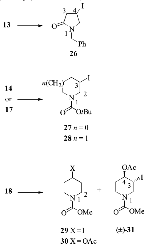
Scheme 6. Synthesis of functionalized pyrrolidines and piperidines by radical decarboxylation of \beta - and \gamma -amino acids; see Table 1 for conditions and yields
