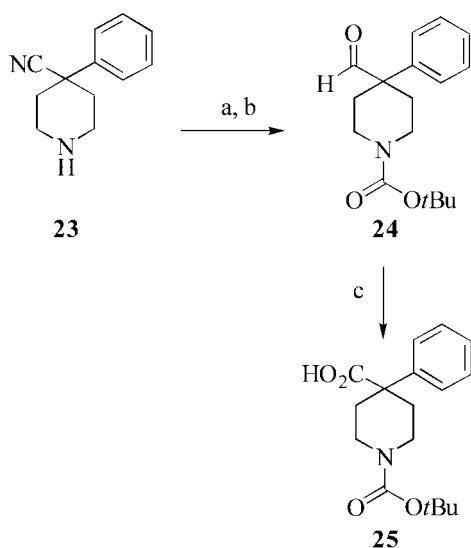
Scheme 5. Synthesis of substrate 25 ; reagents and conditions: (a) [t\text{BuO}(\text{O})\text{C}]_2\text{O} , \text{CH}_2\text{Cl}_2 , \text{Et}_3\text{N} , room temp., 94%; (b) DIBAL-H, toluene, -78^\circ\text{C} , 4 h; then \text{NH}_4\text{Cl} (aq), -78^\circ\text{C} to room temp., 53%; (c) aq. \text{NaH}_2\text{PO}_4 , \text{H}_2\text{O}_2 , aq. \text{NaClO}_2 , MeCN, 95%
