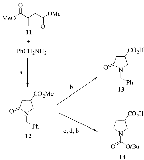
Scheme 3. Synthesis of substrates 13 and 14 ; reagents and conditions: (a) MeOH, reflux, 99%; (b) 2 N NaOH, MeOH, room temp., 85% for 13 , 85% for 14 ; (c) BBN, THF, reflux, 70%; (d) \text{H}_2 , Pd (10 wt.% on C), [\text{tBuO}(\text{O})\text{C}]_2\text{O} , EtOAc, 92%
