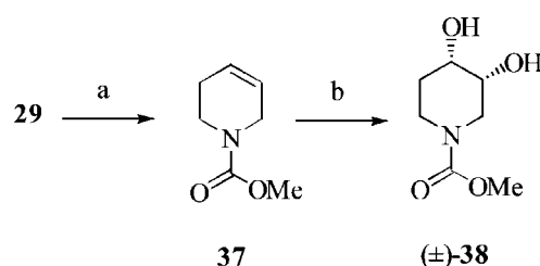
Scheme 8. Synthesis of imino sugar ( \pm )- 38 ; reagents and conditions: (a) DBU, \text{CH}_2\text{Cl}_2 , room temp., 84%; (b) acetone/ \text{H}_2\text{O} (2:1), 0 °C, then \text{OsO}_4 in t\text{BuOH} , NMO, 57%
