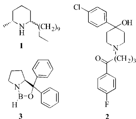
Figure 1. Piperidine and pyrrolidine rings in natural products, synthetic drugs and chiral catalysts
