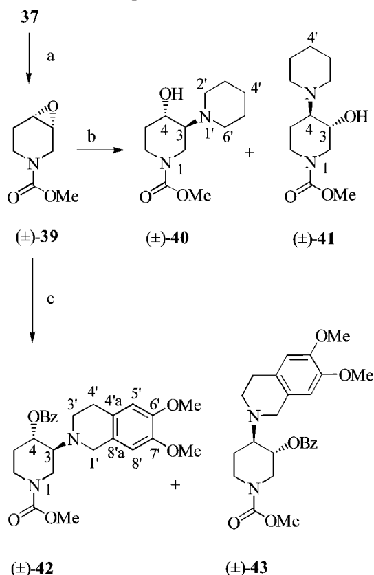
Scheme 9. Synthesis of new antifungal compounds; reagents and conditions: (a) MCPBA, \text{CH}_2\text{Cl}_2 , room temp., 98%; (b) piperidine, EtOH, \text{Et}_3\text{N} , 29% for ( \pm )- 40 , 19% for ( \pm )- 41 ; (c) 6,7-dimethoxy-1,2,3,4-tetrahydroisoquinoline, EtOH, \text{Et}_3\text{N} ; then \text{BzCl} , \text{CH}_2\text{Cl}_2 , \text{Et}_3\text{N} , 35% for ( \pm )- 42 , 16% for ( \pm )- 43
