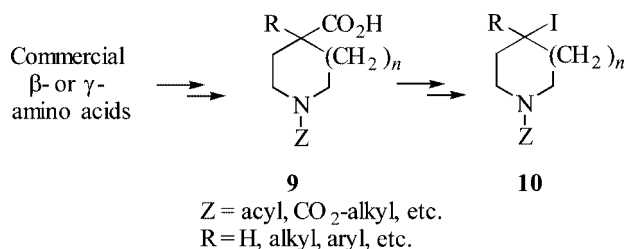
Scheme 2. Synthesis of substituted nitrogen heterocycles from \beta - and \gamma -amino acids
