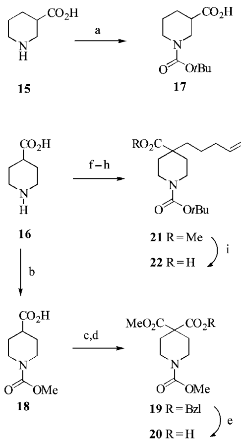
Scheme 4. Synthesis of substrates 17 , 18 , 20 and 22 ; reagents and conditions: (a) [\text{tBuO}(\text{O})\text{C}]_2\text{O} , 1 N aq. NaOH, THF, 91%; (b) \text{ClCO}_2\text{Me} , THF/sat. aq. \text{NaHCO}_3 , 75%; (c) NaI, \text{K}_2\text{CO}_3 , BzI, MeCN, 0 °C to room temp., 79%; (d) LDA, THF, -78 °C; then \text{ClCO}_2\text{Me} in THF, -78 °C to room temp., 94%; (e) \text{H}_2 , \text{Pd}(\text{OH})_2 (20 wt.% on C), EtOAc, room temp., 99%; (f) \text{SOCl}_2 , MeOH, -12 °C to room temp.; (g) \text{CH}_2\text{Cl}_2 , \text{Et}_3\text{N} , (\text{BOC})_2\text{O} , DMAP (cat.), 79% for the two steps; (h) LDA, THF, -78 °C; then 5-bromo-1-pentene, -78 °C to room temp., 78%; (i) 2 N NaOH, MeOH, reflux, 87%
